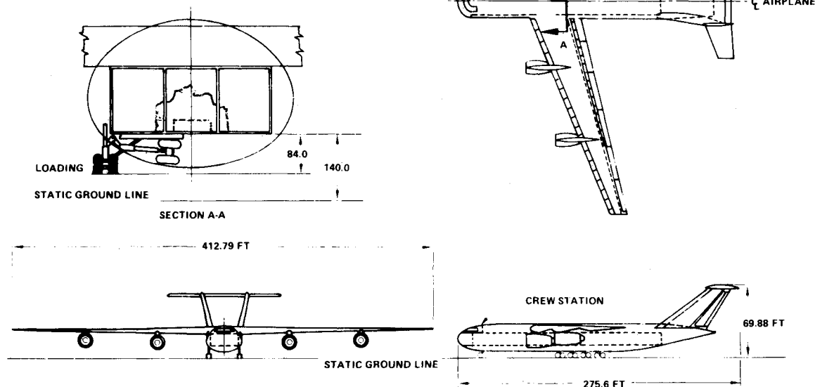
Fig. 2 Reference turbulent airplane.
