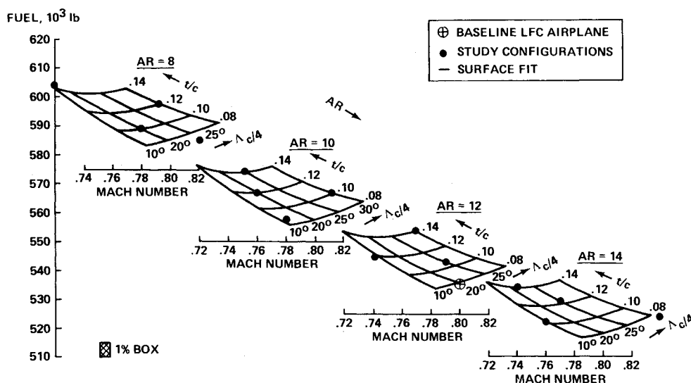
Fig. 6 Effect of wing planform geometry on fuel.
