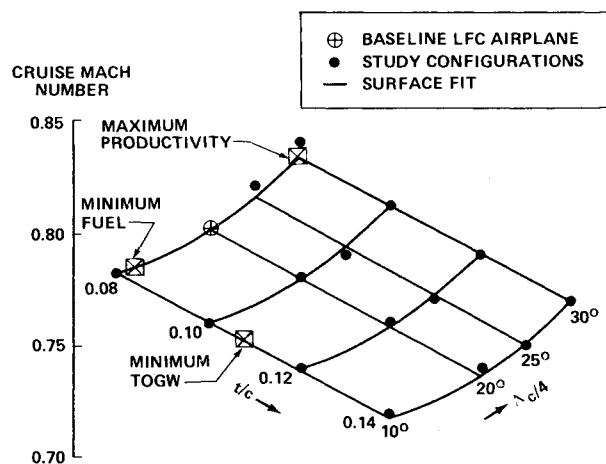
Fig. 5 Effect of wing planform geometry on cruise Mach.
