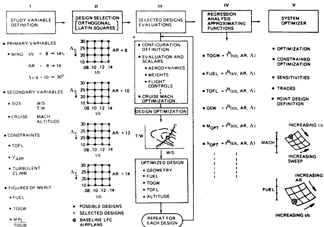
Fig. 4 Laminar flow control wing parametric optimization study.
