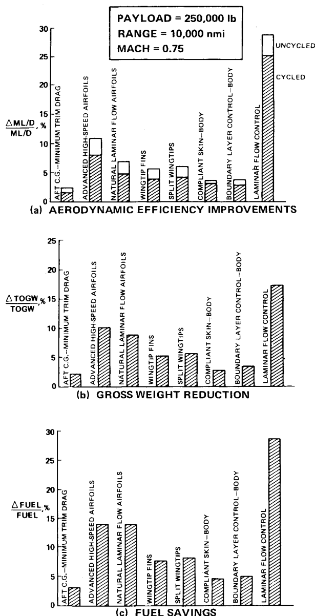
Fig. 1 Potential benefits of advanced aerodynamic concepts.
