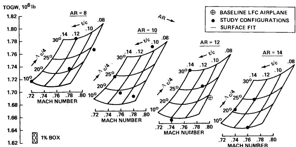
Fig. 7 Effect of wing planform geometry on weight.
