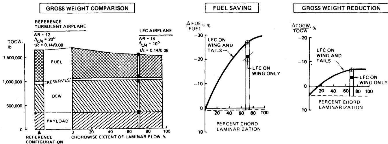
Fig. 10 Effect of extent of laminarization on fuel and weight.
