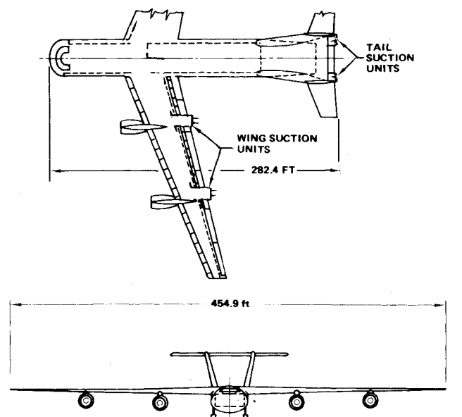
Fig. 8 Final laminar flow control airplane.
